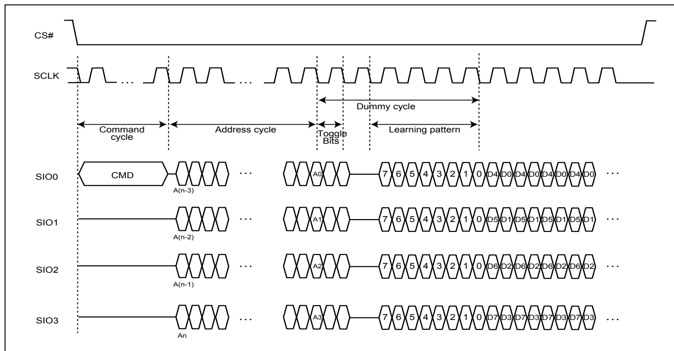
Figure 52. DTR4IO (DC=6)
