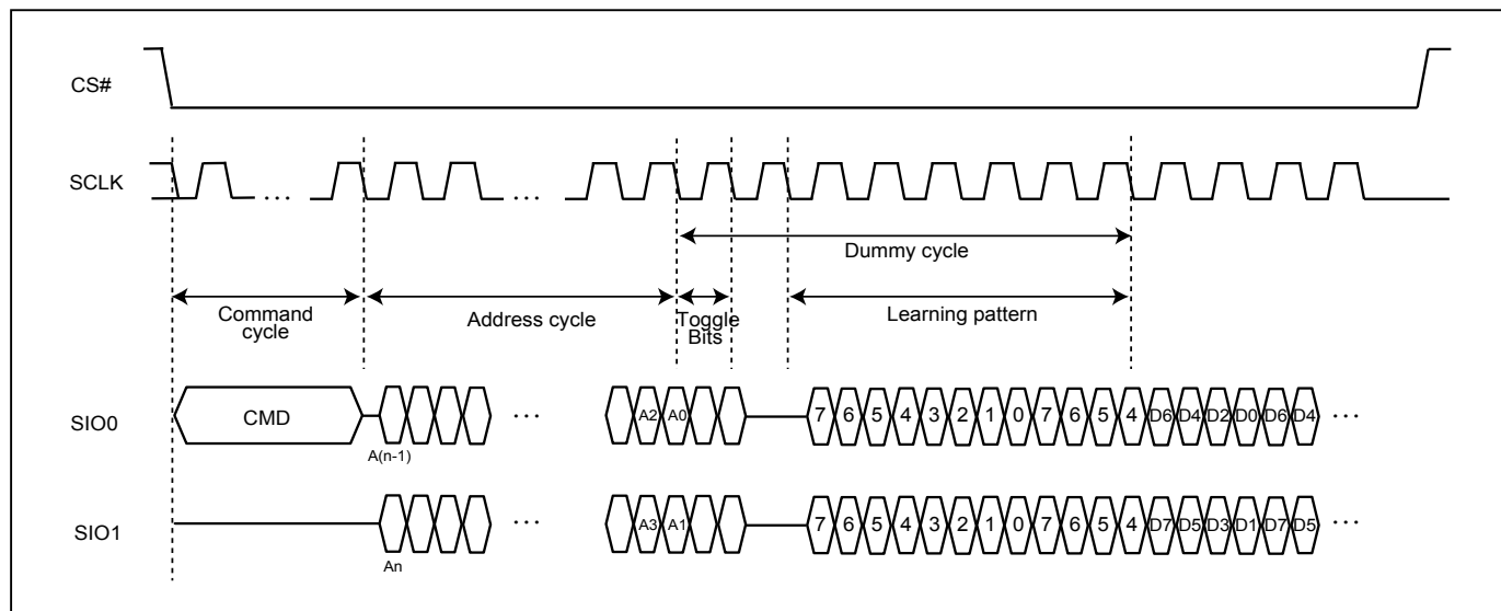
Figure 51. DTR2IO (DC=8)
