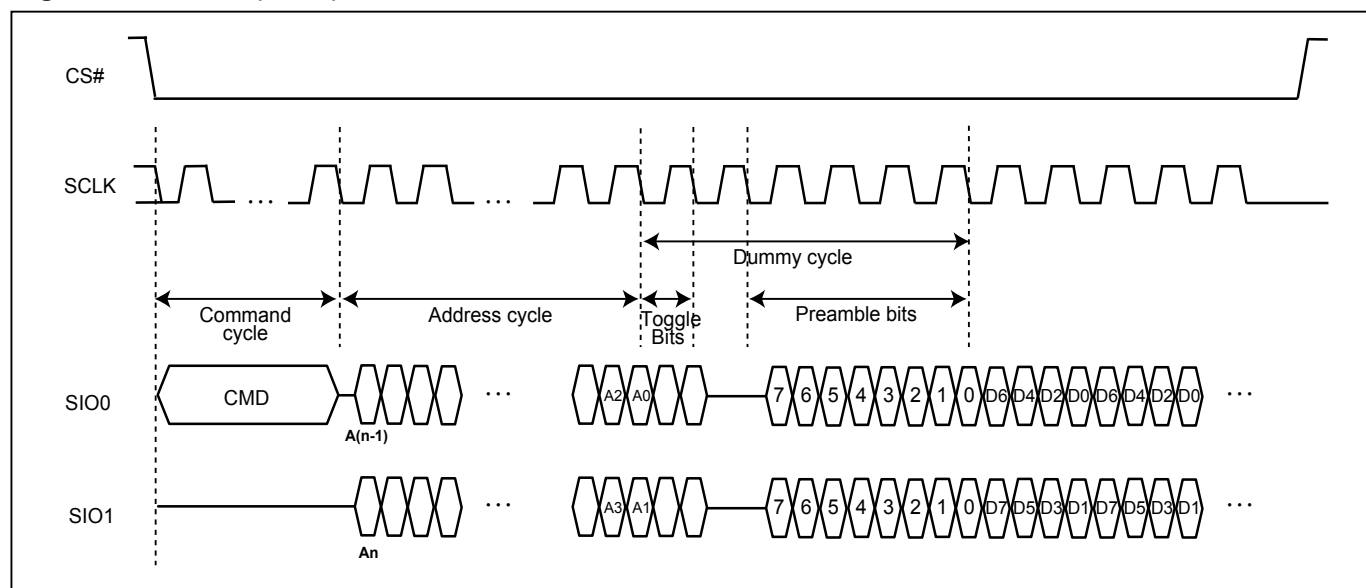
Figure 50. DTR2IO (DC=6)
