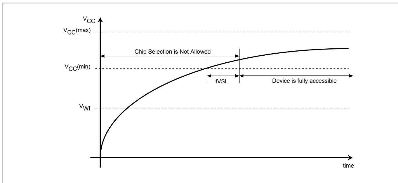
Figure 118. Power-up Timing
