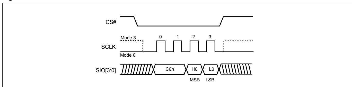
Figure 71. QPI Mode
