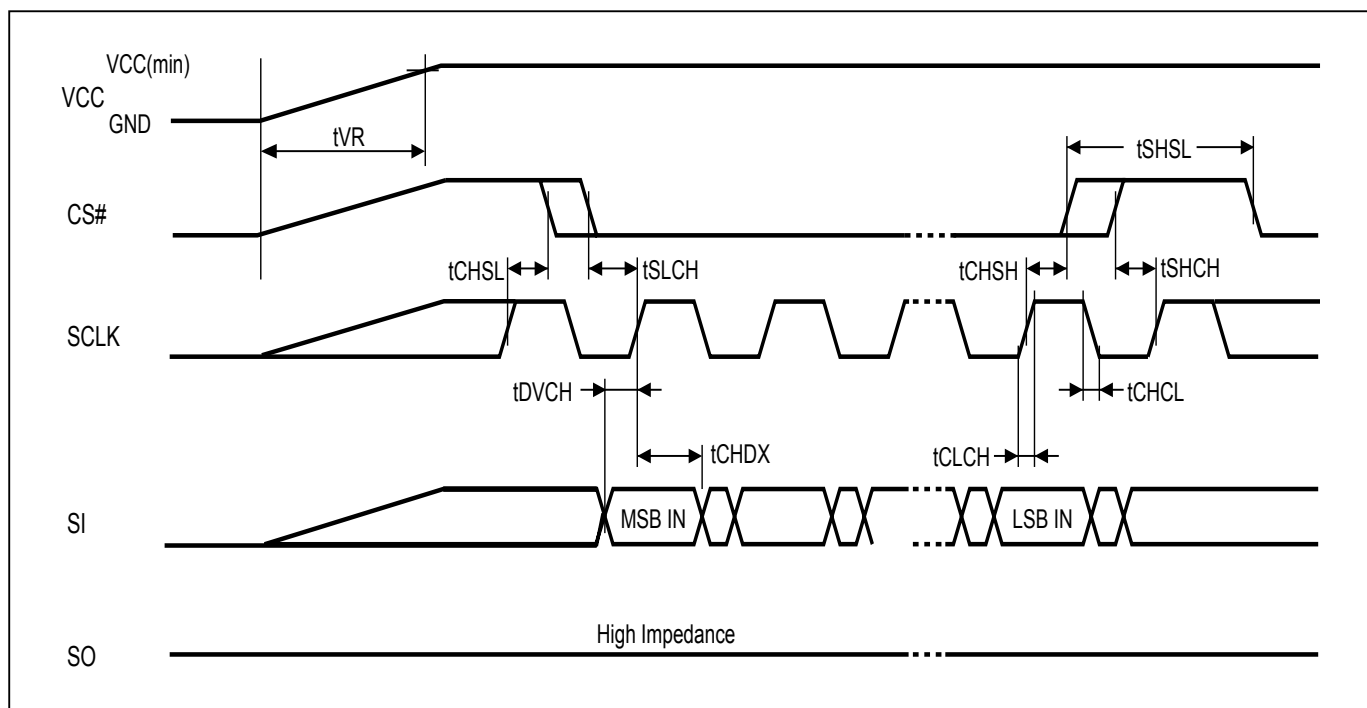
Figure 116. AC Timing at Device Power-Up
