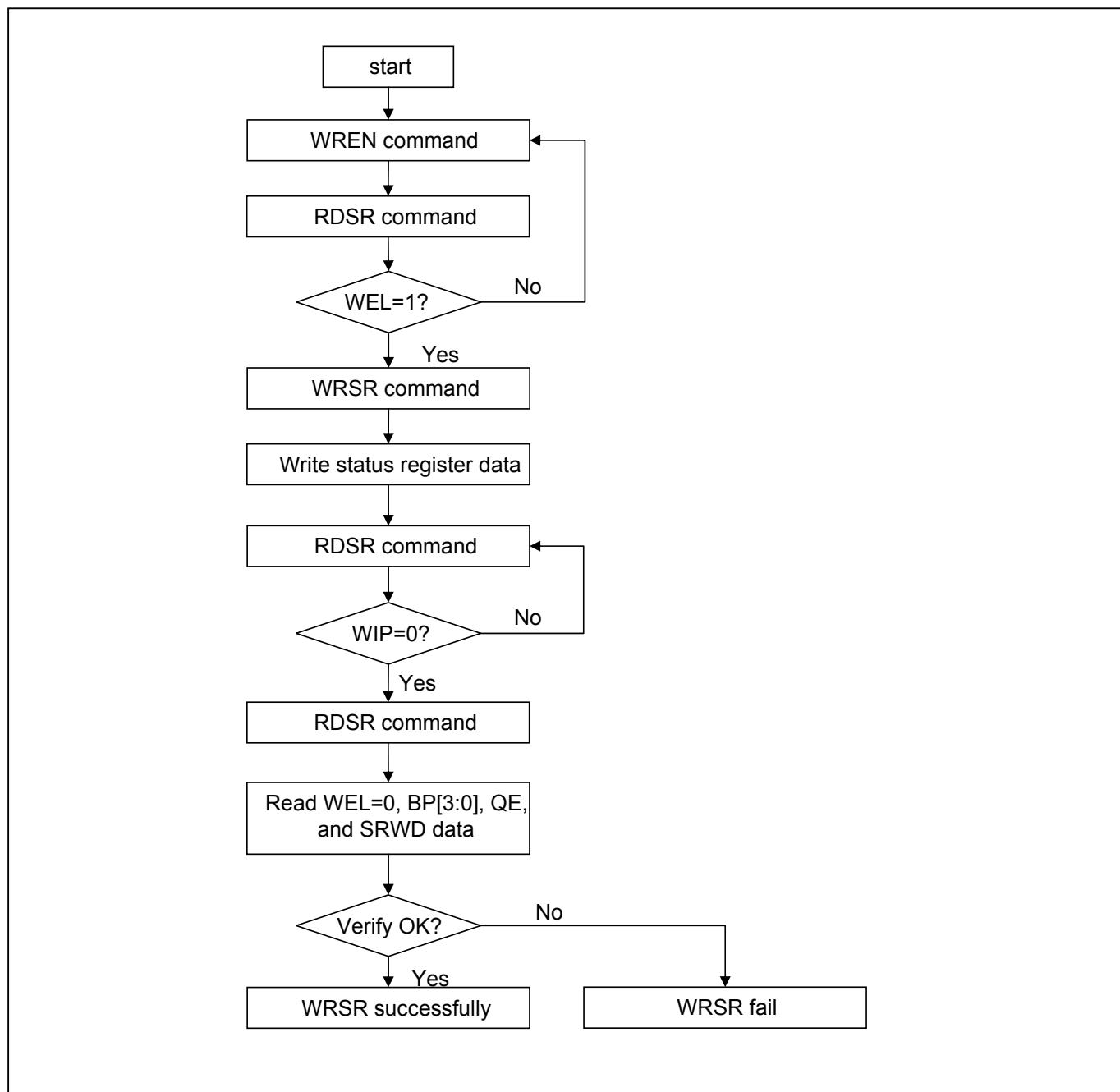
Figure 30. WRSR flow
