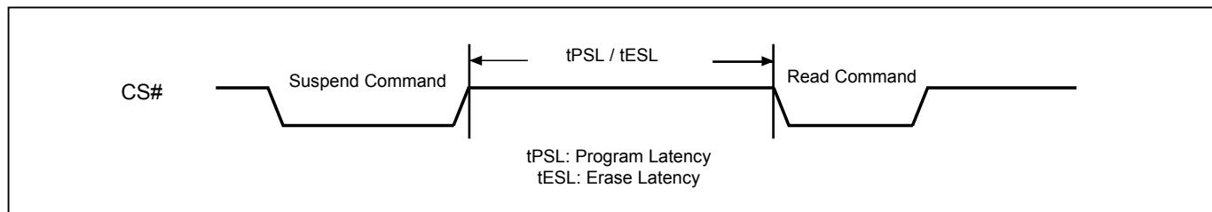
Figure 104. Suspend to Read Latency
