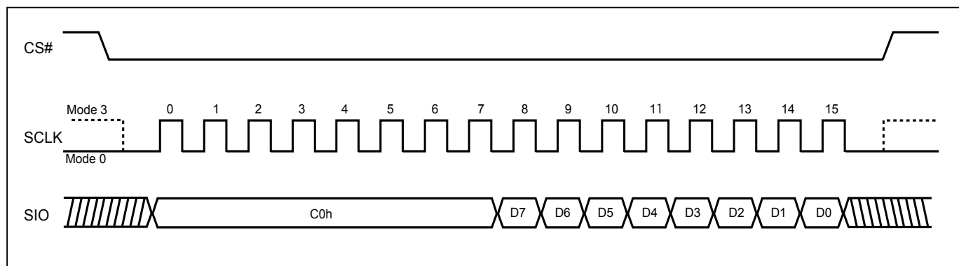
Figure 70. SPI Mode
