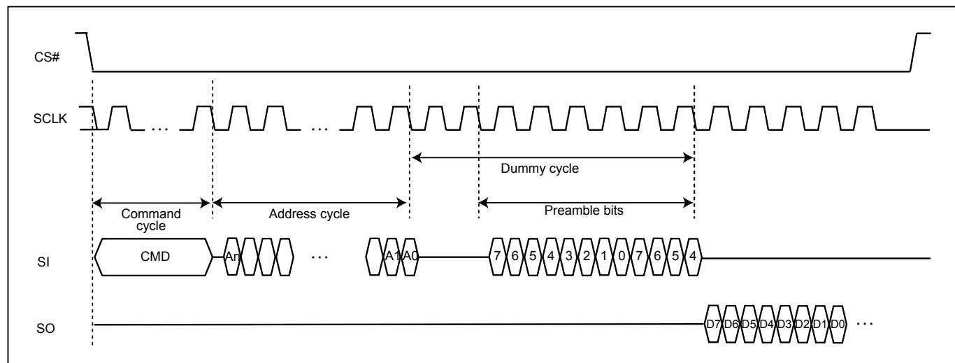
Figure 49. DTR1IO (DC=8)
